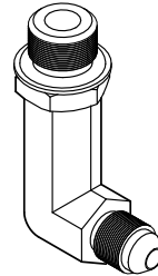
5550008 FTG ELB -04JIC -06 ORB x 43mm
