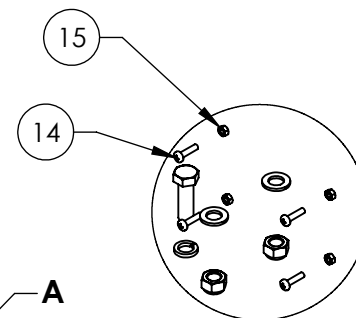
DETAIL D SCALE 1 : 8
