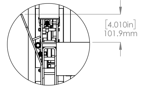
DETAIL A SCALE 1 : 8
