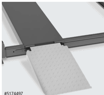
Aluminum Approach Ramps Width - 19.75" / Length - 36.75"
