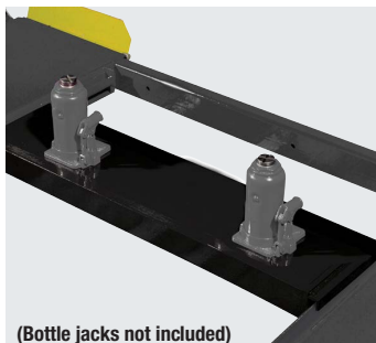
JP-6 Telescoping #5175349 6,000 lb. Capacity Jack Platform
